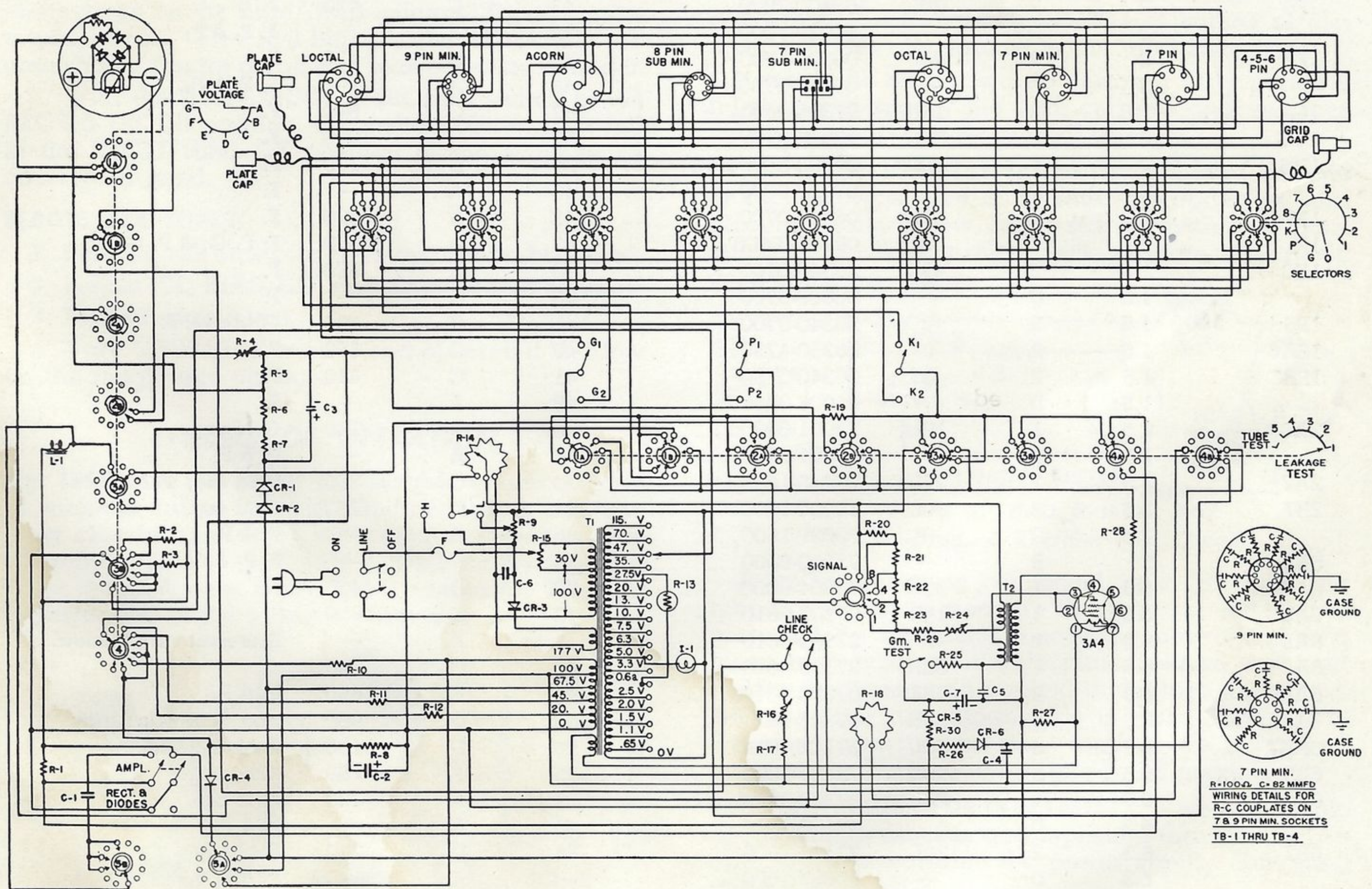
Schematic Wiring Diagram — Model 981 Type 3
