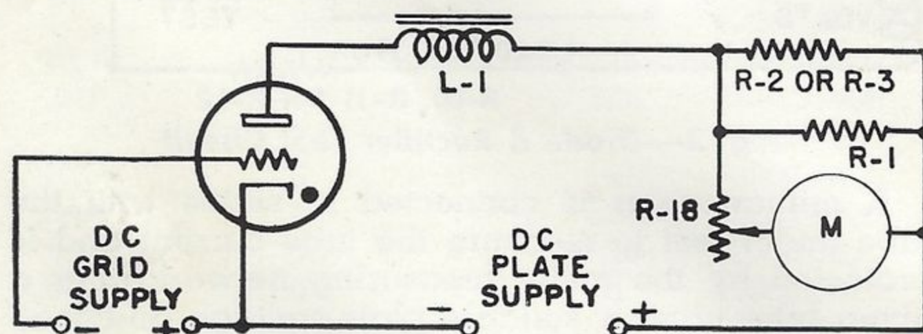
Fig. 5—Thyratron Test Circuit
