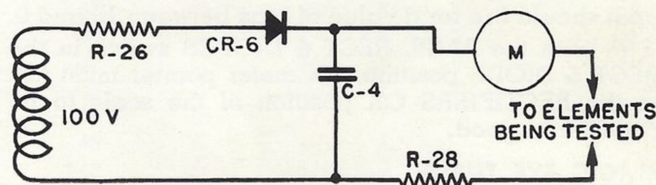
Fig. 6—Leakage Test Circuit
