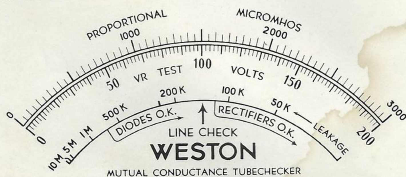
Fig. 1—Actual Size Scale—Model 981 Type 3
