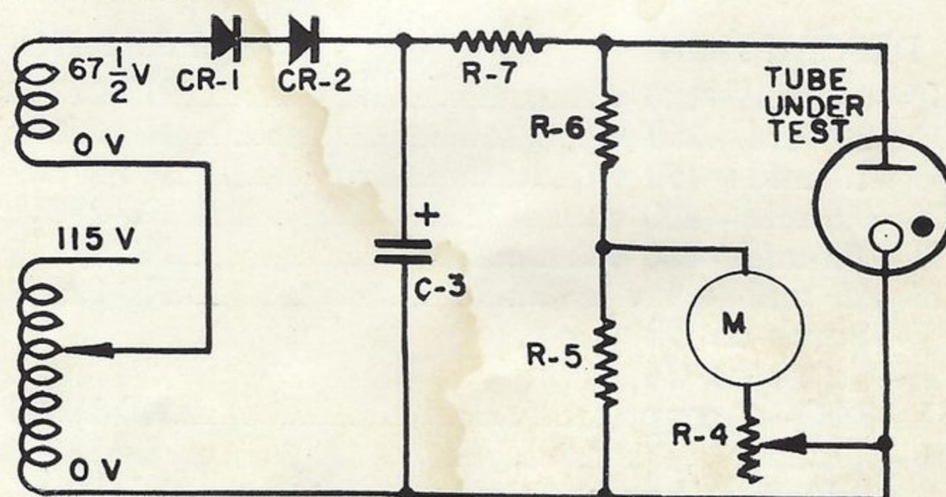
Fig. 4—Voltage Regulator Test Circuit
