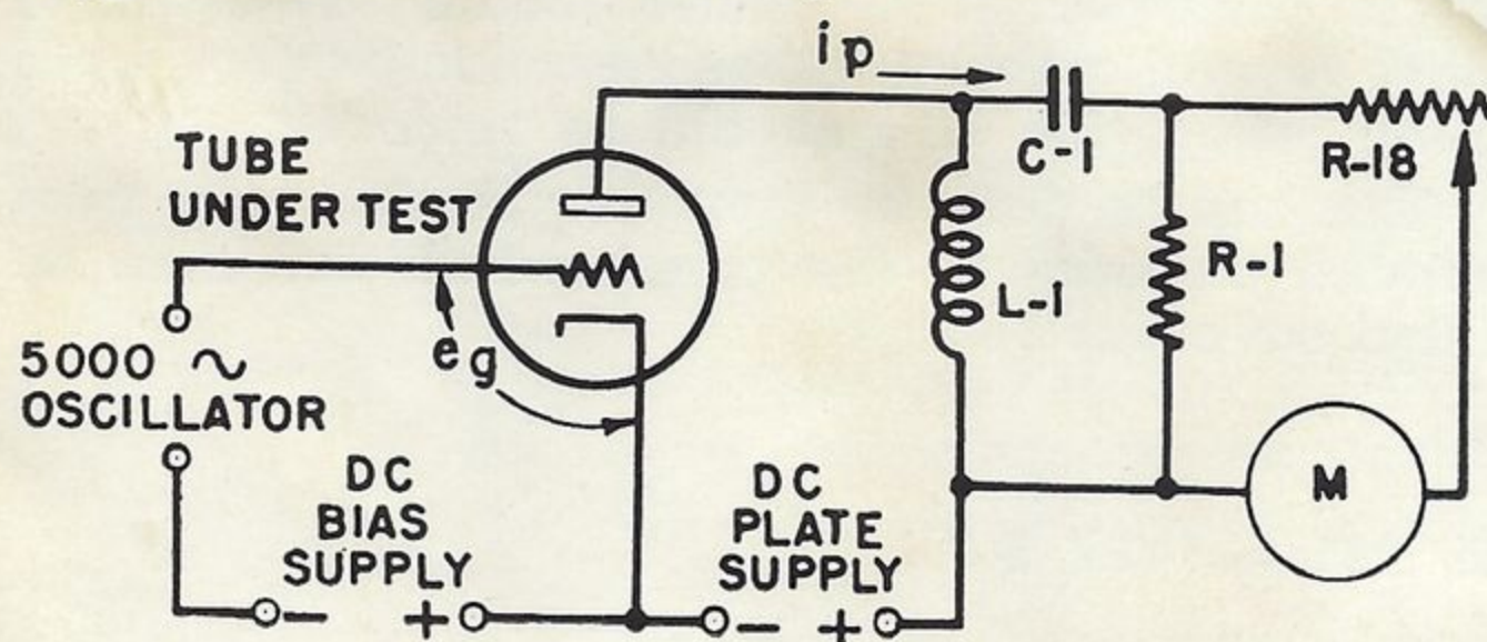
Fig. 2—Basic Gm Test Circuit
